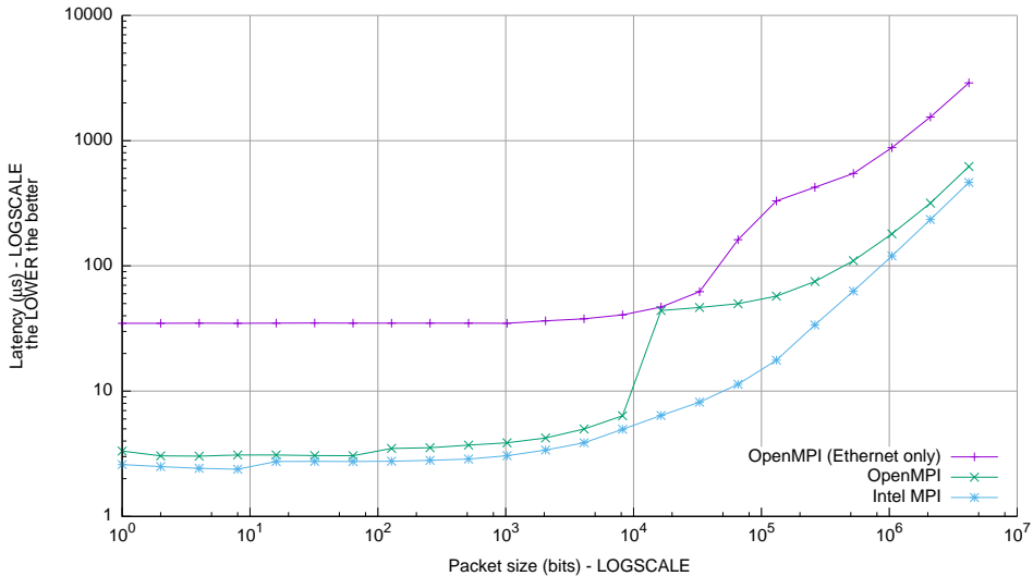
OSU One Sided MPI Get latency Test v5.3.2
