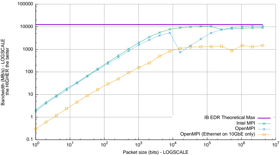
OSU MPI One Sided MPI Get Bandwidth Test v5.3.2
